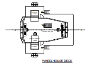
WHEELHOUSE DECK
