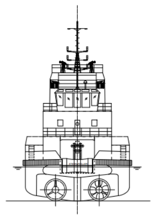
STERN VIEW
