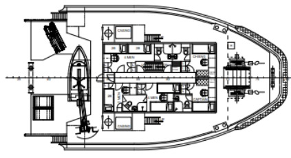
FORECASTLE DECK
