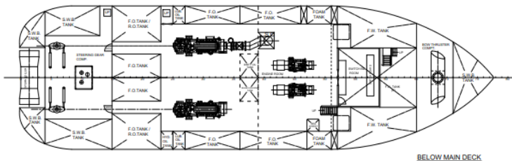
BELOW MAIN DECK
