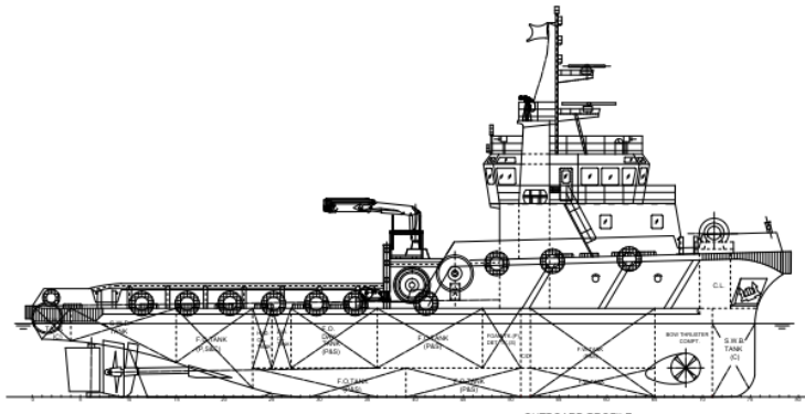
OUTBOARD PROFILE
