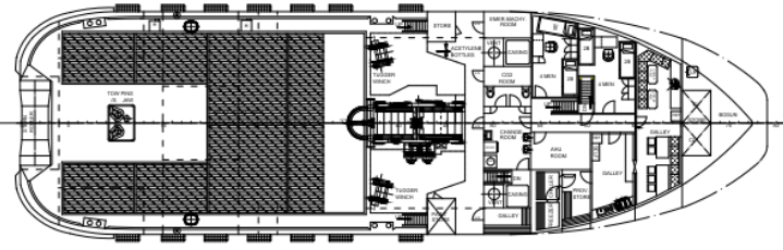
MAIN DECK PLAN
